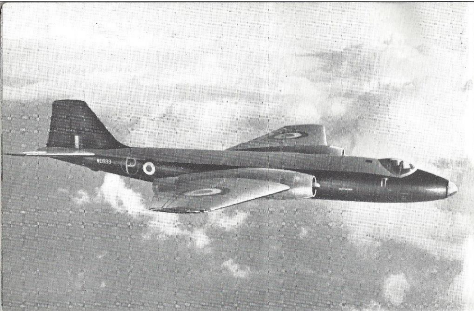
Armstrong Siddeley Sapphire-Canberra experimental version of the Canberra fitted with two Armstrong Siddeley Sapphire Sa.7 jet engines. Another experimental version has Bristol Olympus jet engines. The standard Canberra has Rolls-Royce Avons
