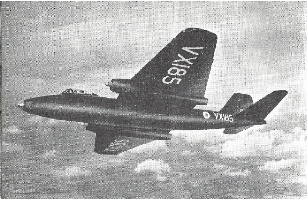
English Electric Canberra B.8 2-seat night intruder version of the Canberra bomber powered by two Rolls-Royce Avon jet engines
