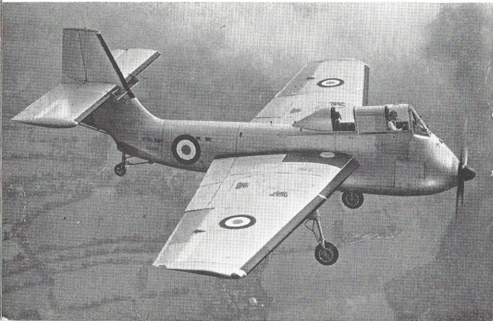
Short Seamew 2-seat carrier-borne anti-submarine search and strike aircraft powered by an Armstrong Siddeley Mamba turboprop engine
