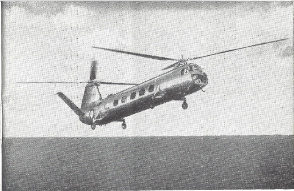
Bristol Type 173 13-seat helicopter powered by two Alvis Leonides piston engines
