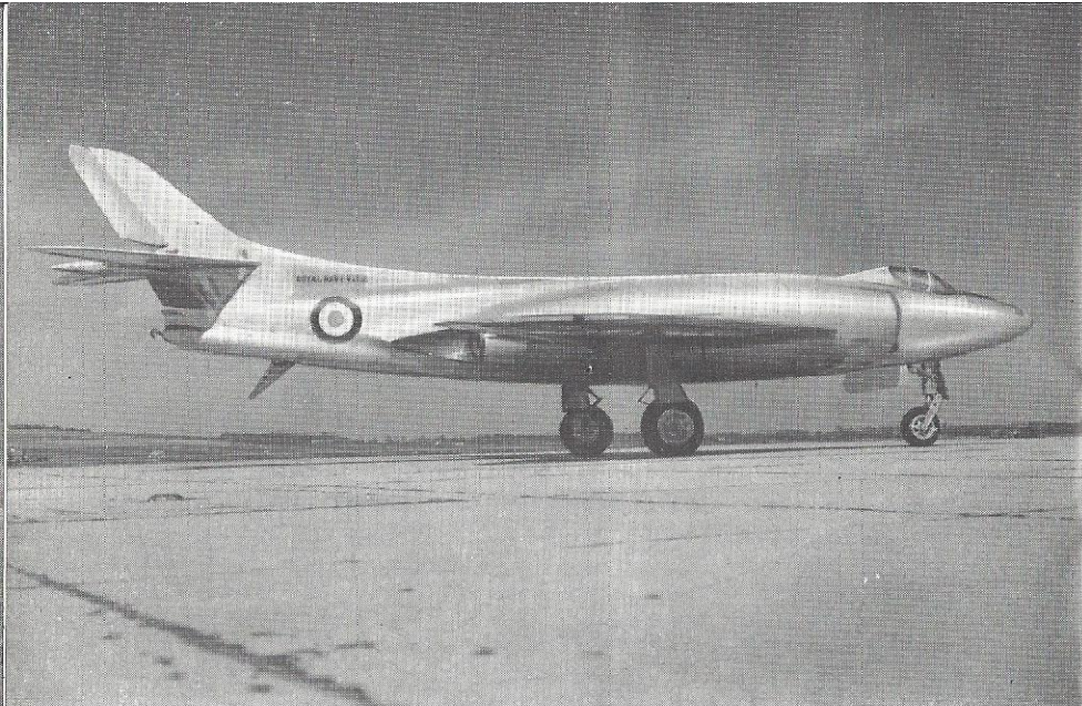
Vickers Supermarine Type 525 single-seat experimental carrier-borne naval fighter powered by two Rolls-Royce Avon jet engines
